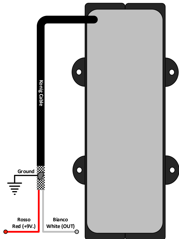
Cable connection
