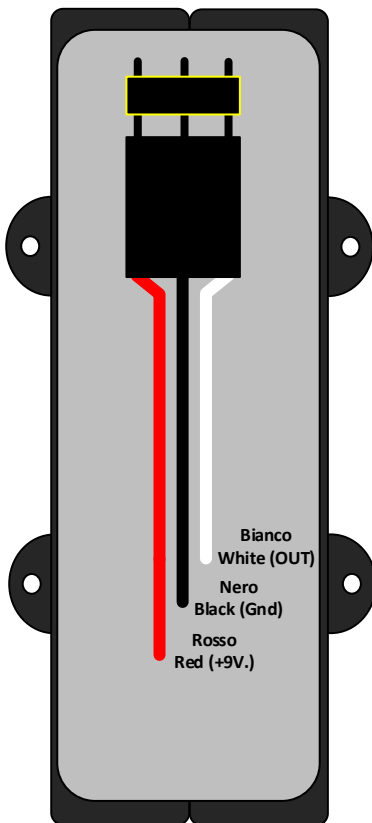
Quick connection
